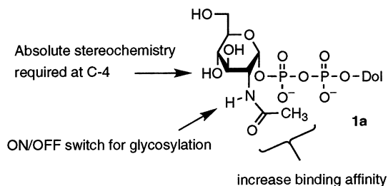
Figure 4. Substrate specificity of glycosyl acceptor for Enzyme II.
